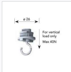
N047210 SUSPENSION HOOK
